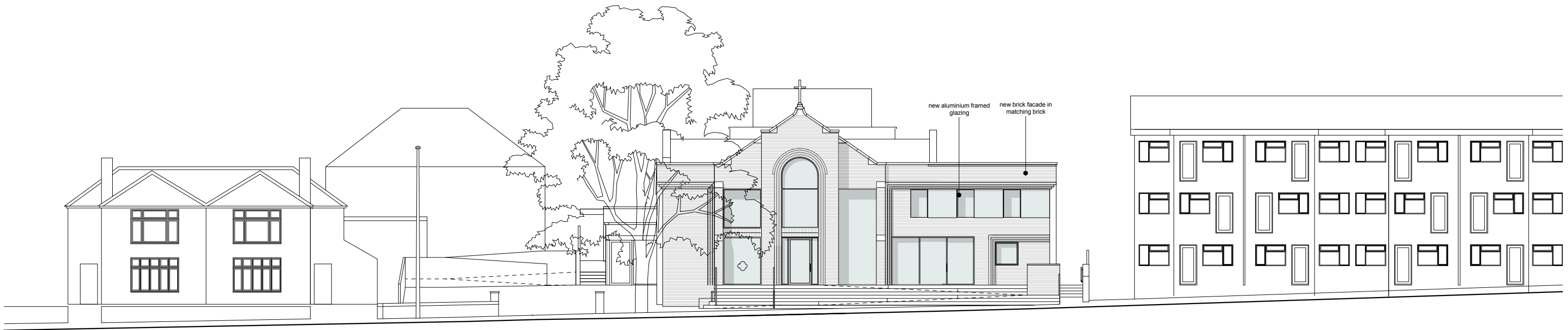
01 | JOEL STREET ELEVATION scale 1:200
